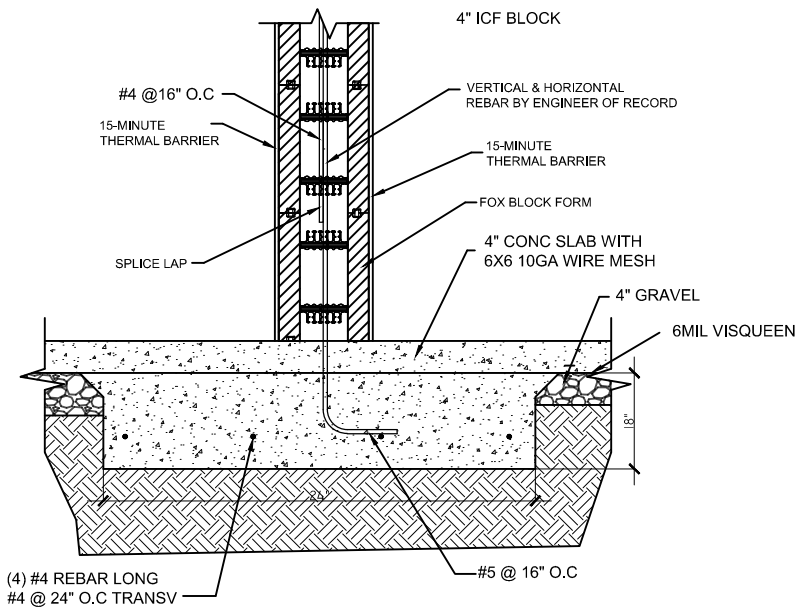
INT FOUNDATION DETAIL SCALE 1/2"=1'-0"
