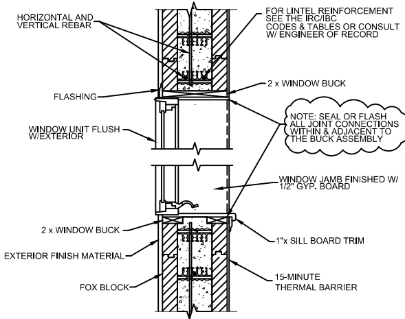
WINDOW HEAD/SILL DETAIL SCALE NTS
