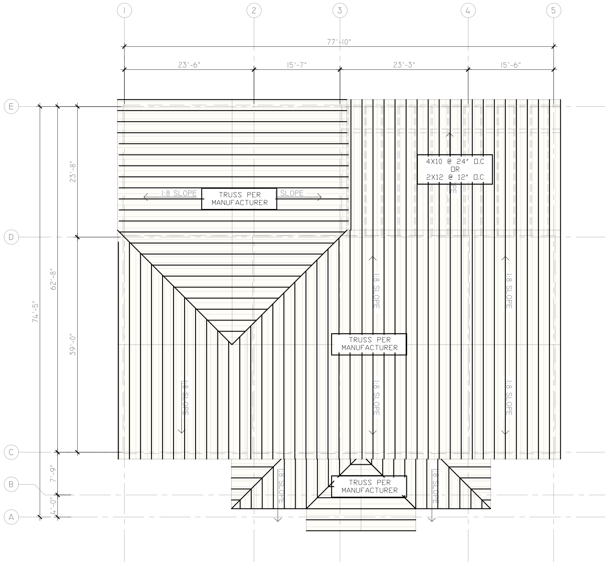
ROOF PLAN SCALE 3/32"=1'-0"
