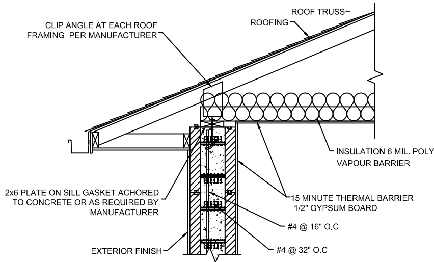
WALL TO ROOF DETAIL SCALE NTS
