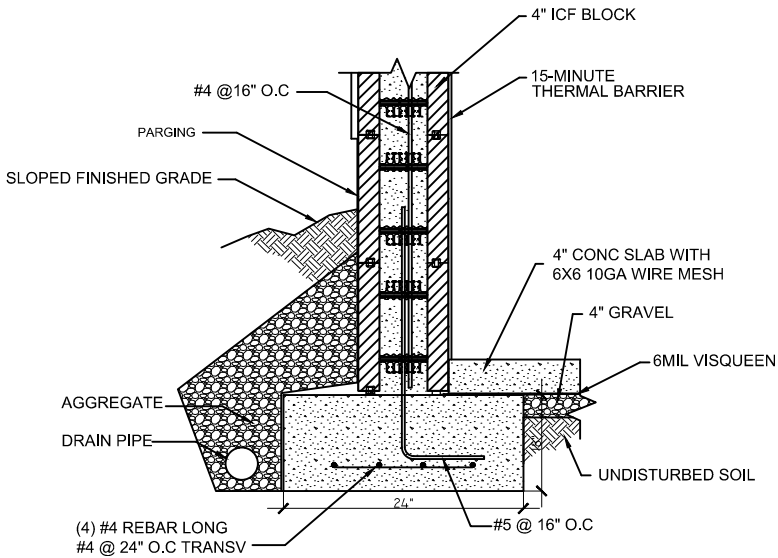
EXT FOUNDATION DETAIL SCALE 1/2"=1'-0"
