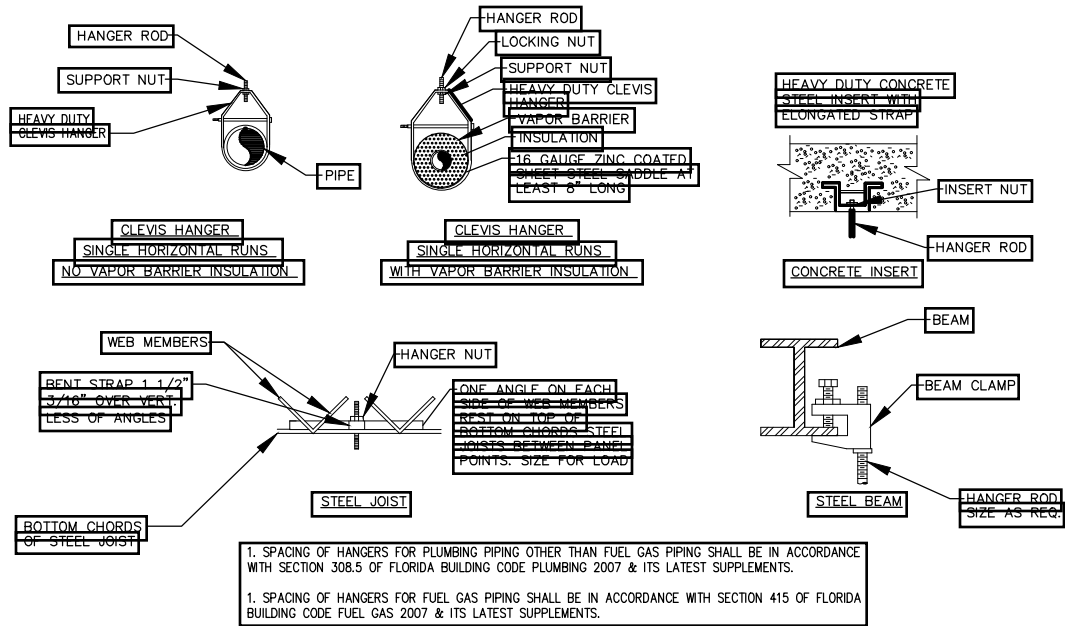
4 PIPE SUPPORTS DETAILS NTS
