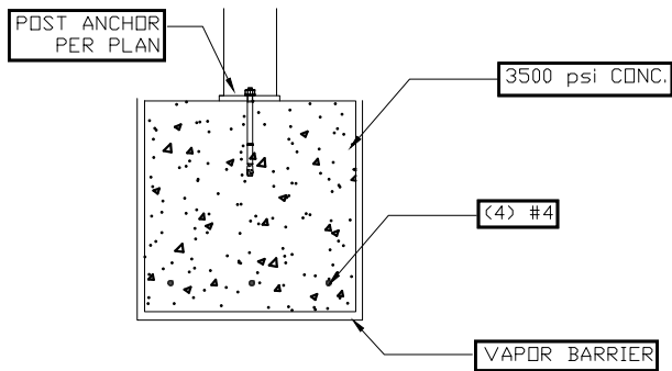
WOOD POST DETAIL SCALE 1/2"=1'-0"
