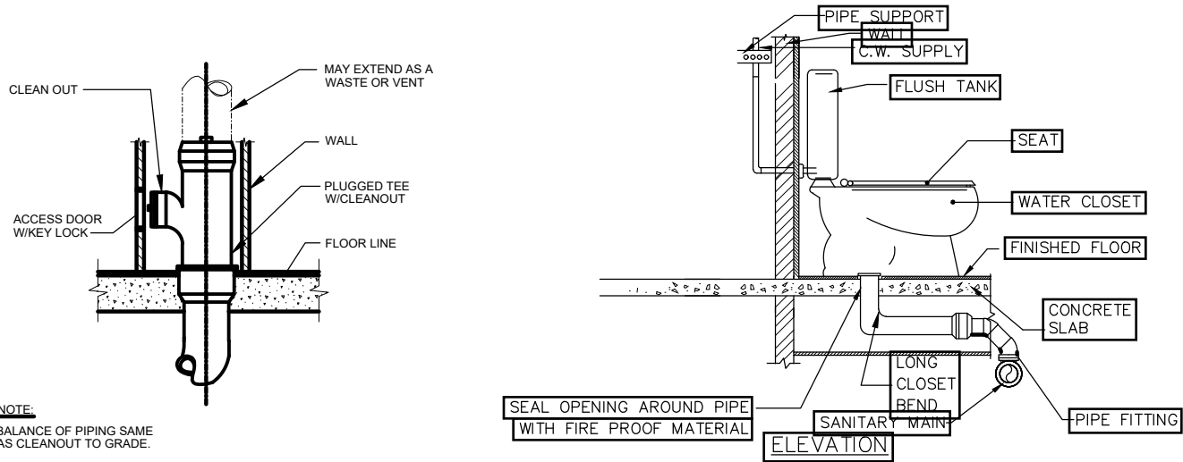
1 WALL CLEANOUT DETAIL NTS
